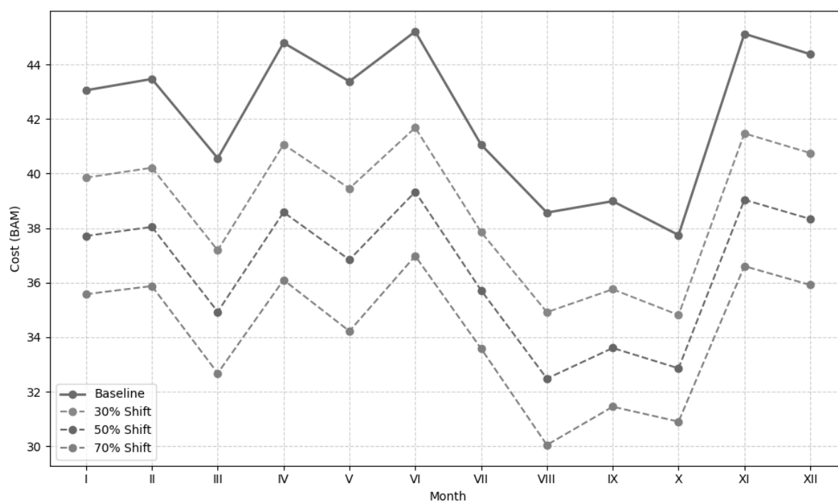
Figure 3. Monthly electricity cost: Basic vs. load shifting
