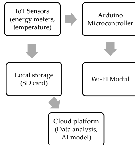
Figure 1. Simulated hardware architecture for smart energy optimization prototype Source: authors
