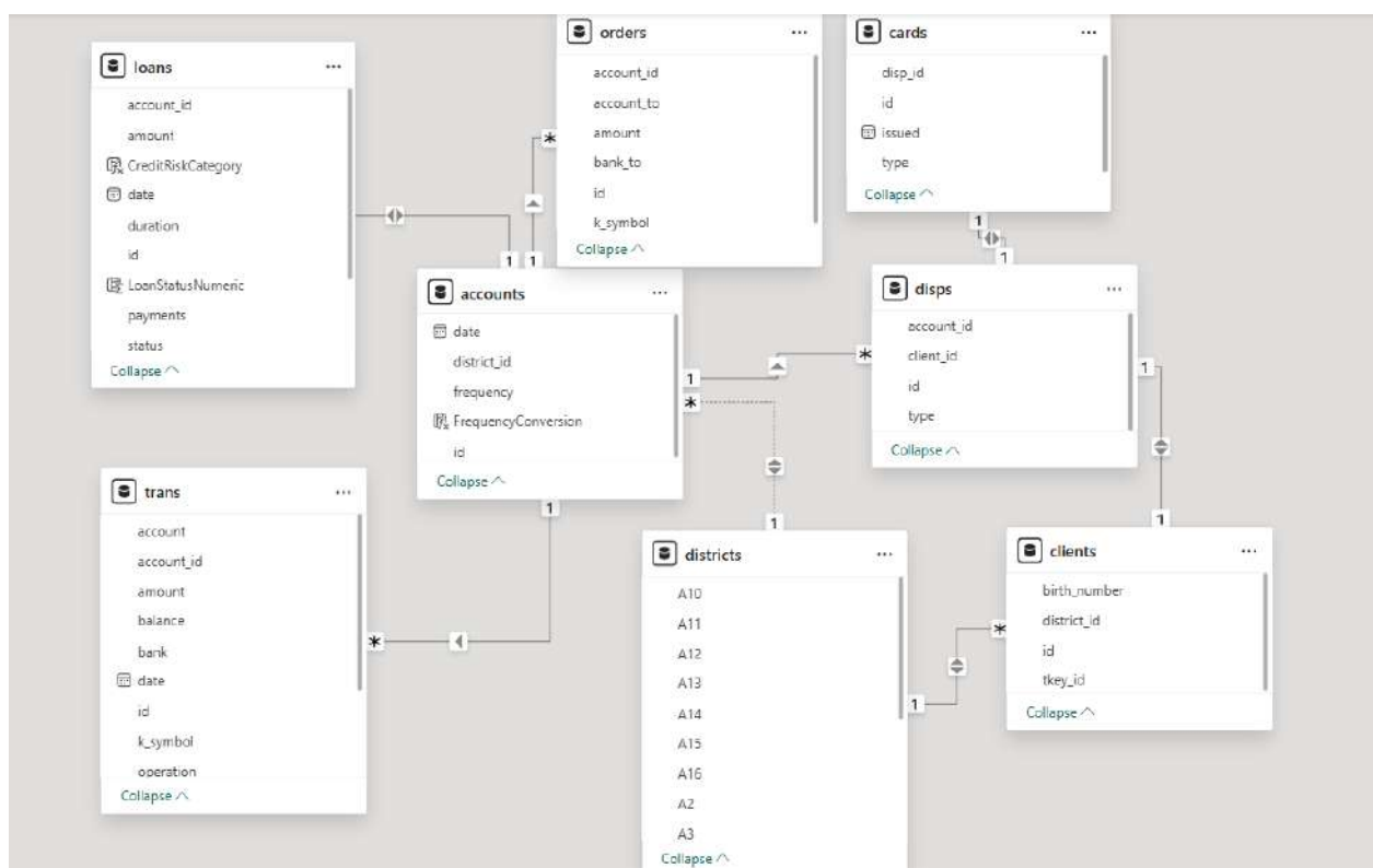
Figure 2. Overview of the dataset with all tables and relationships in the Power BI tool
