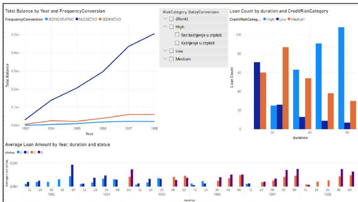
Figure 5. Visualization of dataset results before prediction
