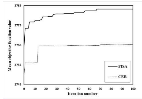
Figure 1. Convergence curves for the FISA and CER on the image Tree (red, k = 12 )
