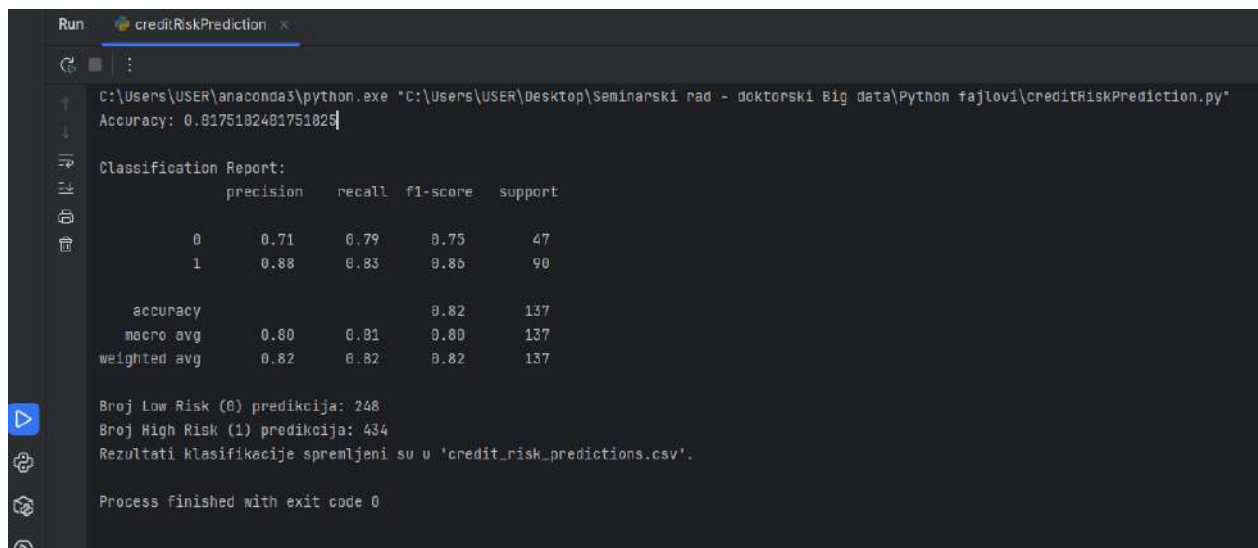
Figure 4. Display of DecisionTreeClassifier algorithm results with a model accuracy of 0.82 (82%)
