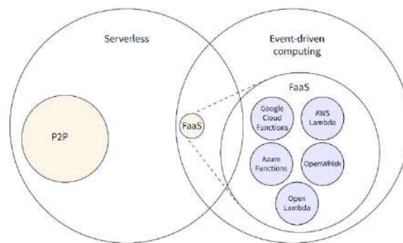
Figure 1. Serverless computing and FaaS
