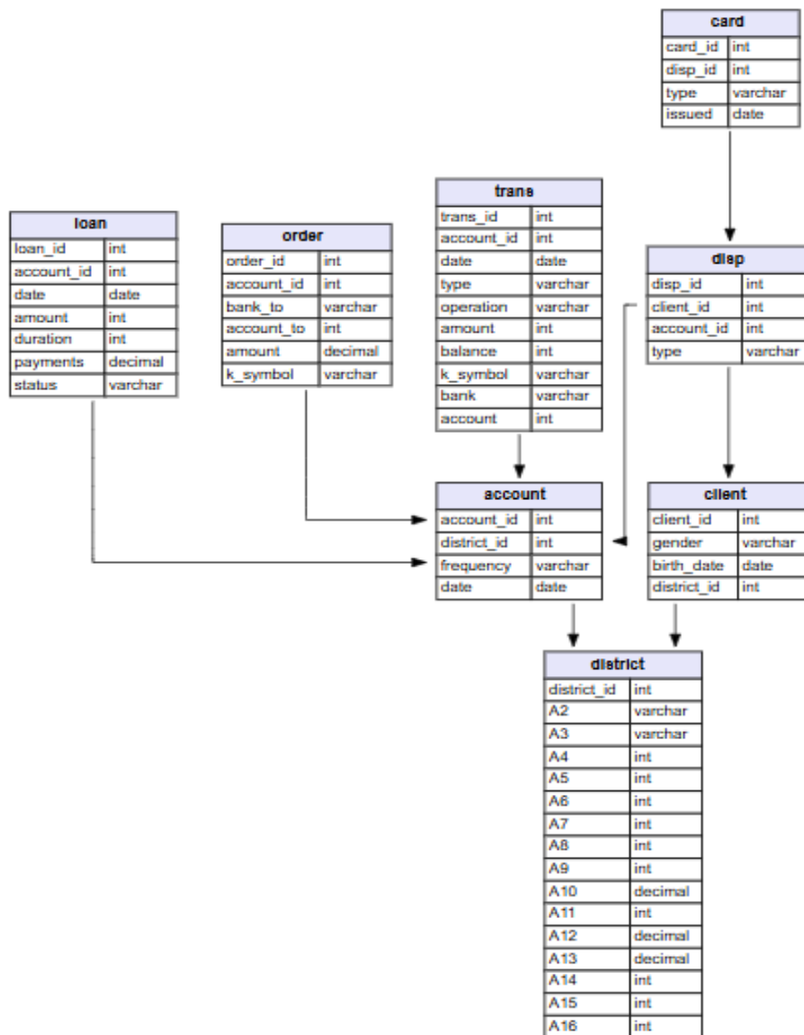
Figure 1. Structure of the Financial dataset showing credit transactions and related tables Source: Berka, 1999
